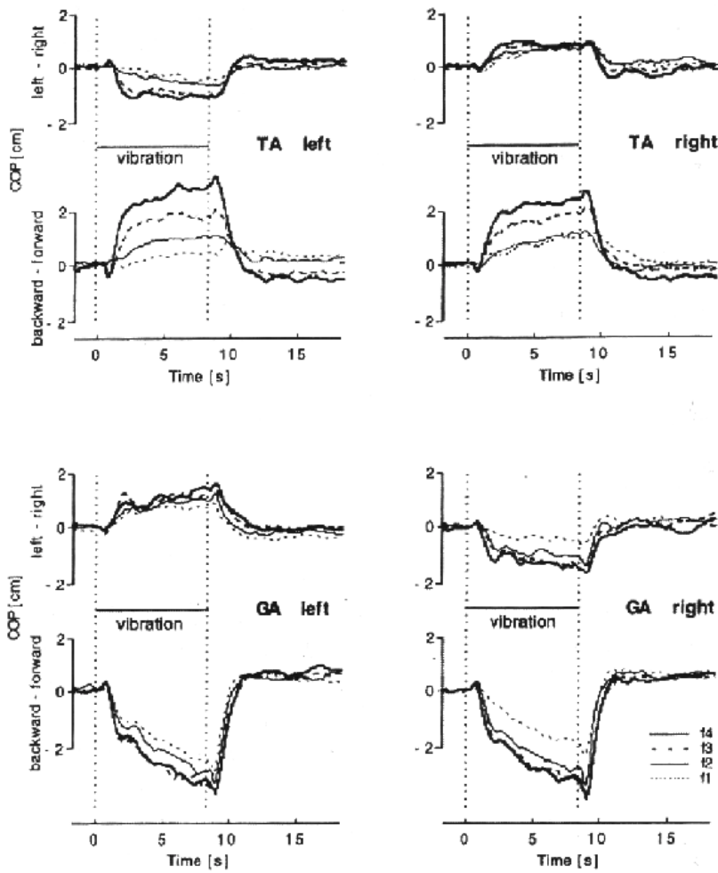
Fig. 1. Forward-backward and left-right time records (CoP) of grand average postural responses of all subjects to different vibration frequencies. The oriented body tilts evoked by vibration were dependent on the muscle stimulated (TA or GA). Body tilt magnitude depended on the frequency and increased from f_1 (40 Hz) to f_4 (100 Hz).
